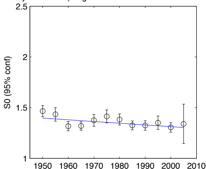
5-year blocks (S0 gradient = -0.001687 \pm 0.000985 )
