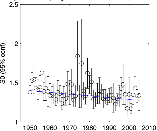
1-year blocks (S0 gradient = -0.002272 \pm 0.000944 )
