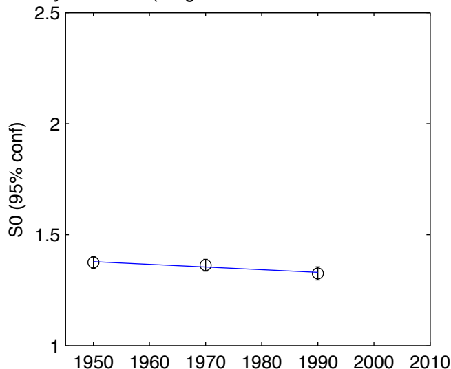
20-year blocks (S0 gradient = -0.001196 \pm 0.000979 )
