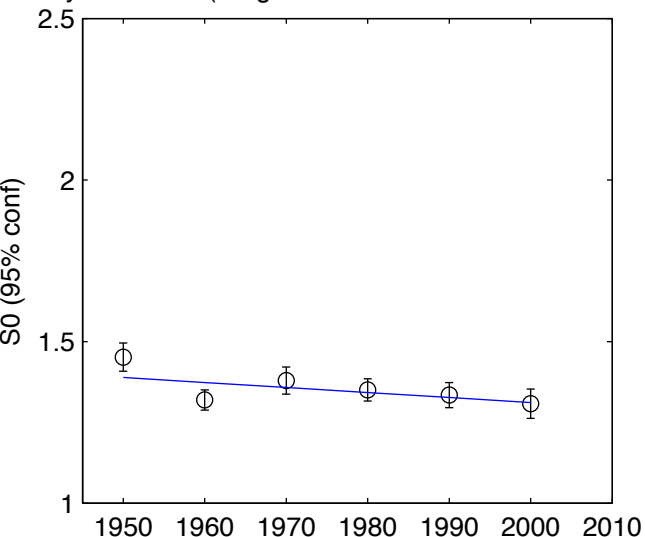
10-year blocks (S0 gradient = -0.001543 \pm 0.000980 )
