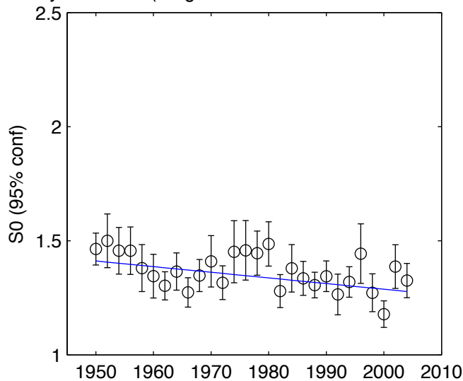
2-year blocks (S0 gradient = -0.002477 \pm 0.000948 )
