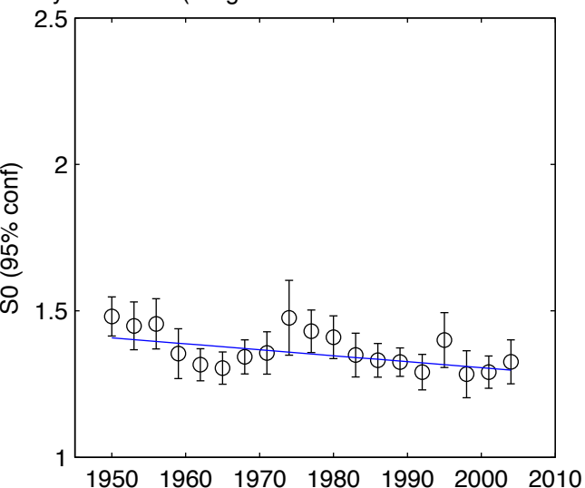
3-year blocks (S0 gradient = -0.002036 \pm 0.000959 )
