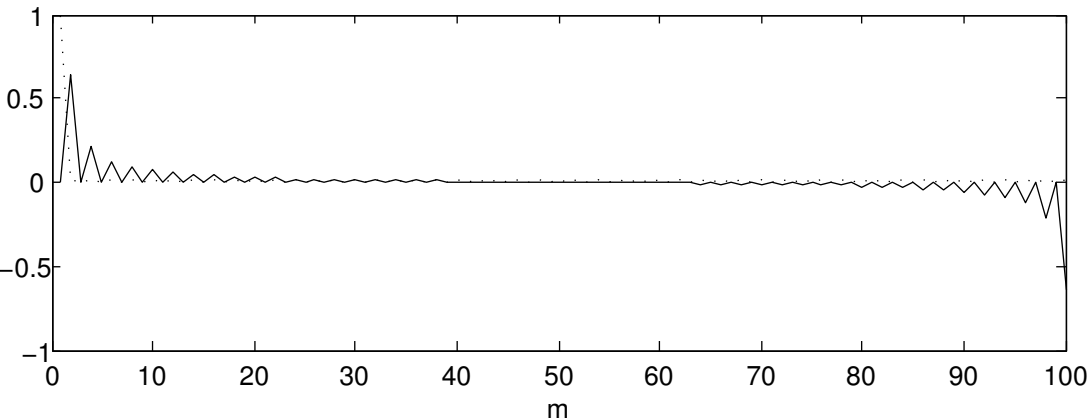
fourier transform
