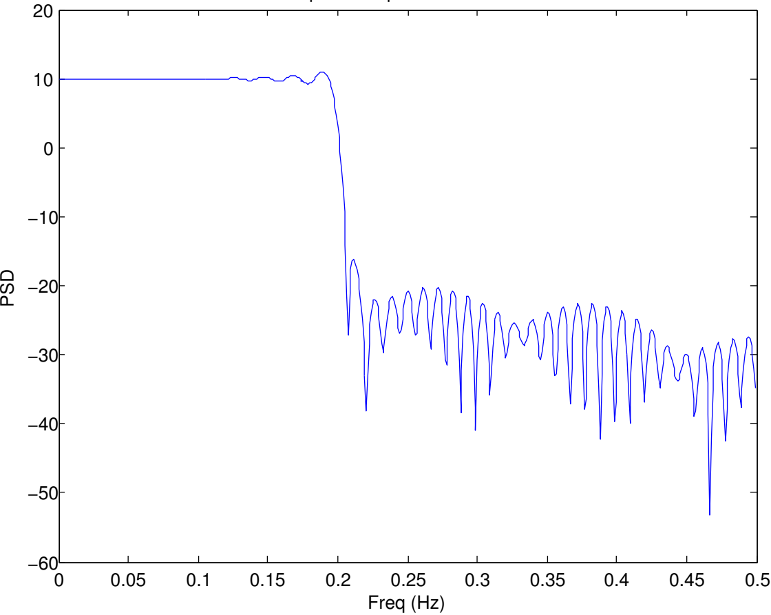
Interpolated Spectrum of a Pulse
