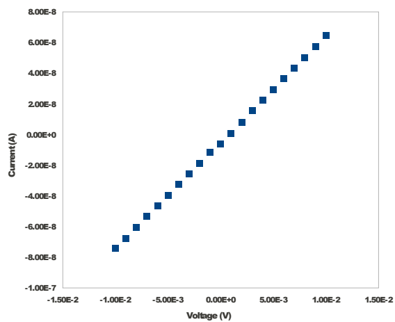
(a) I-V curve for quartz-carrier mounted Si nanowire, 2010-07-01. Resistance is about 155k \Omega .
