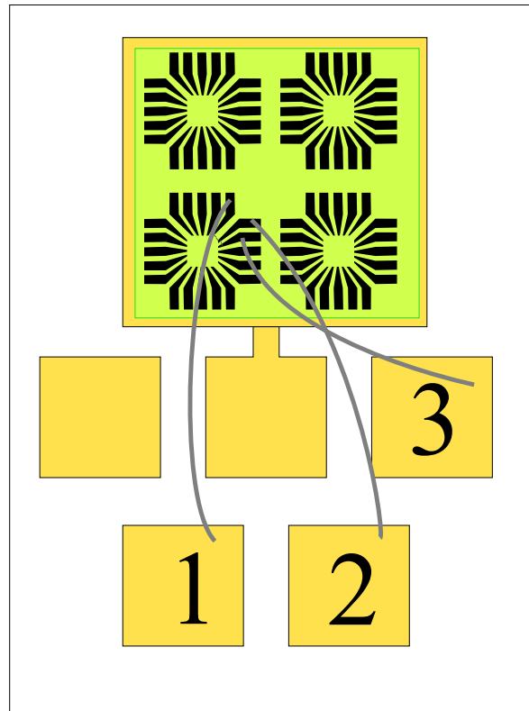
(b) A sketch of the quartz-carrier device. The nanowire is connected between pads 1 and 2.
