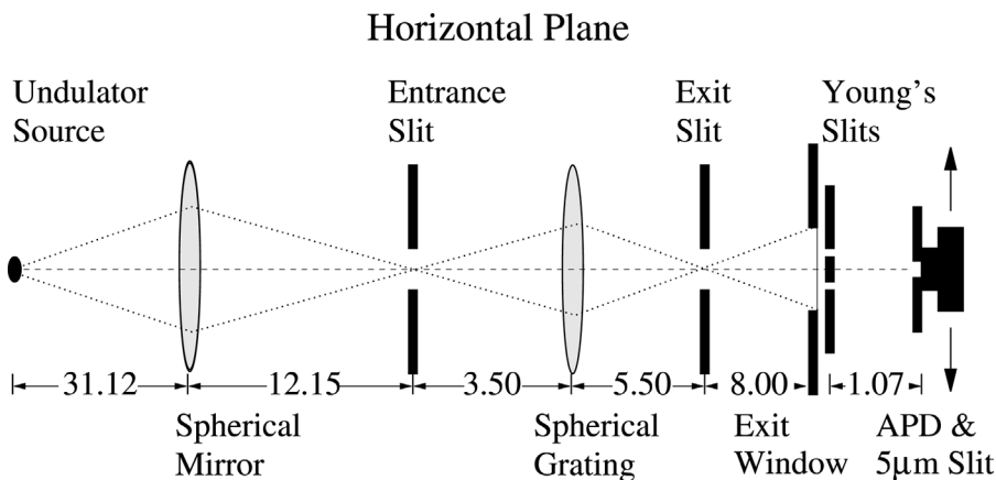
Fig. 1. The 2-ID-B beamline at the Advanced Photon Source showing beamline optics depicted as thin lenses in the horizontal planes. Distances shown are in metres. Distance from the exit slit to the experiment was 8.0 m and from the distance from the undulator source to the exit slit was 52.3 m. The Young’s slits were placed 10 mm downstream of the beamline exit window which is 700 \mu\text{m} \times 700 \mu\text{m} . The detector was an APD with 5 \mu\text{m} slit placed directly in front of the detector window.
